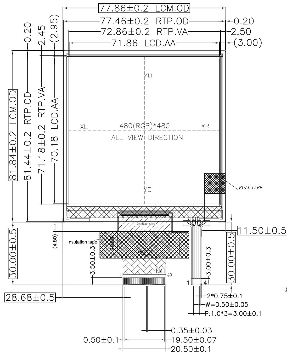
(Front View)
