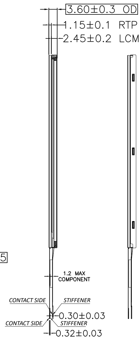
(Side View)
