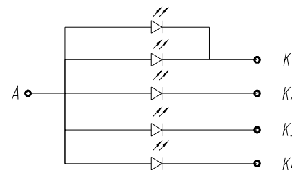
LED Source(CIRCUIT DIAGRAM)
