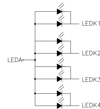
LED CIRCUIT DIAGRAM
